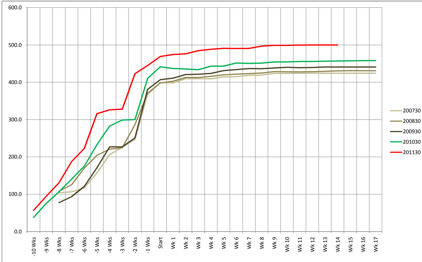
Spring Term FTE Comparison 2007 - 2011 04/28/11
